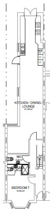
Ground Floor Proposed 1 : 100
